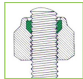
Bolt being driven into Greer Nut
